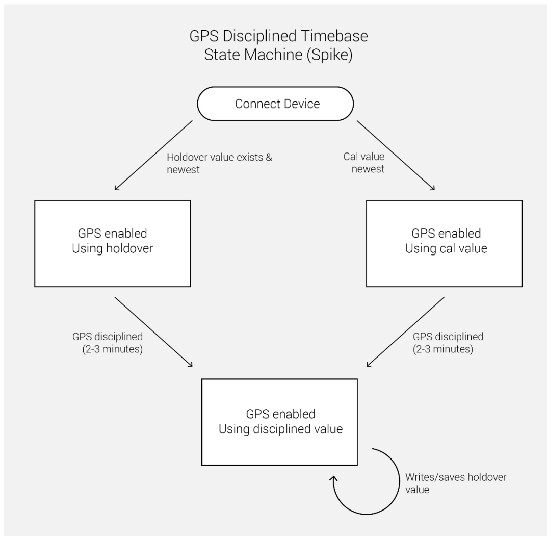
Figure 62: State machine for GPS disciplining for the SM200.
