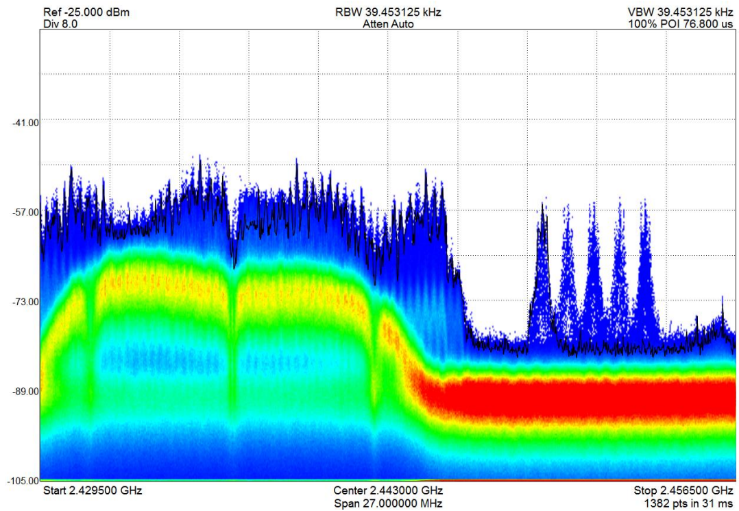
Figure 68: Real-time persistence display of a wireless router and Bluetooth headset coexisting in the ISM band.
