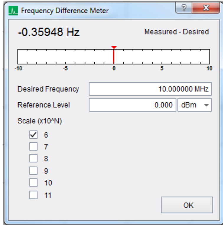
Figure 57: Frequency difference meter observing frequency difference between two 10MHz oscillators
