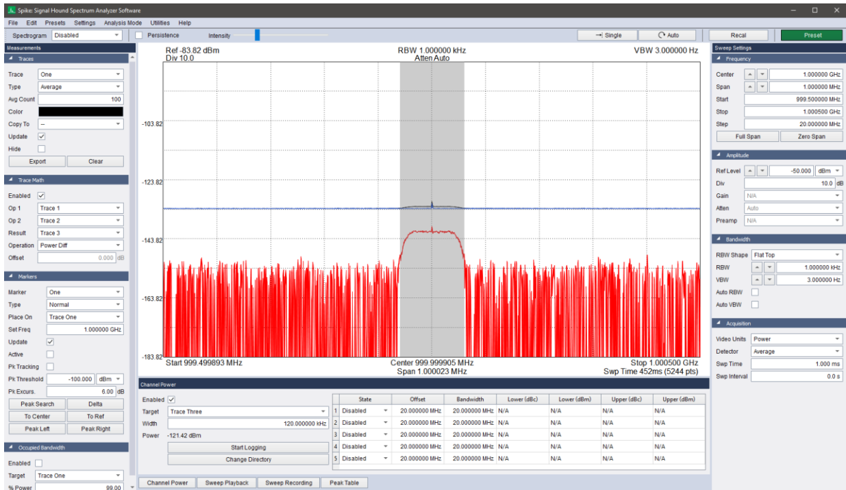
Figure 51: Power difference function measuring signal power below the instrument noise floor.
