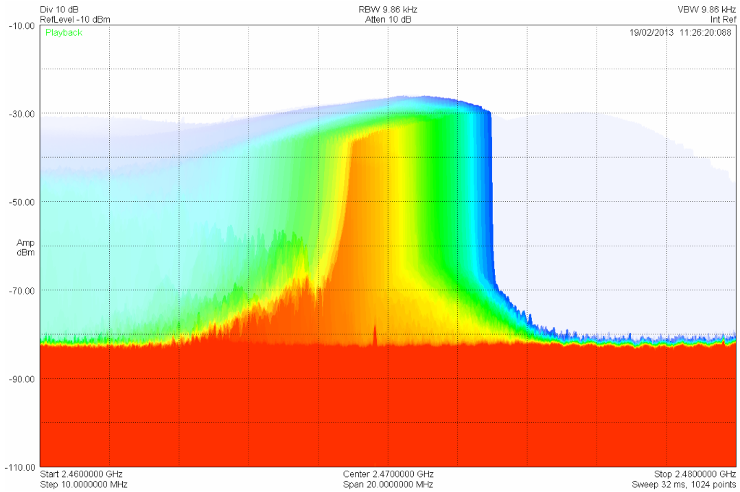
Figure 67: Sweep mode persistence showing the signal from a poorly shielded commercial microwave oven.
