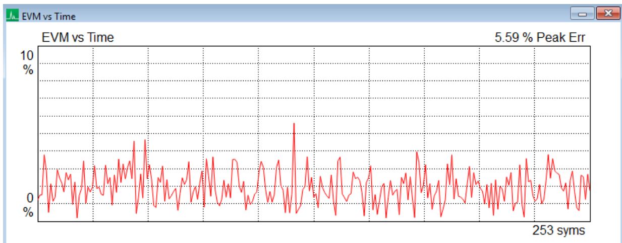
Figure 21 : EVM vs Time plot
