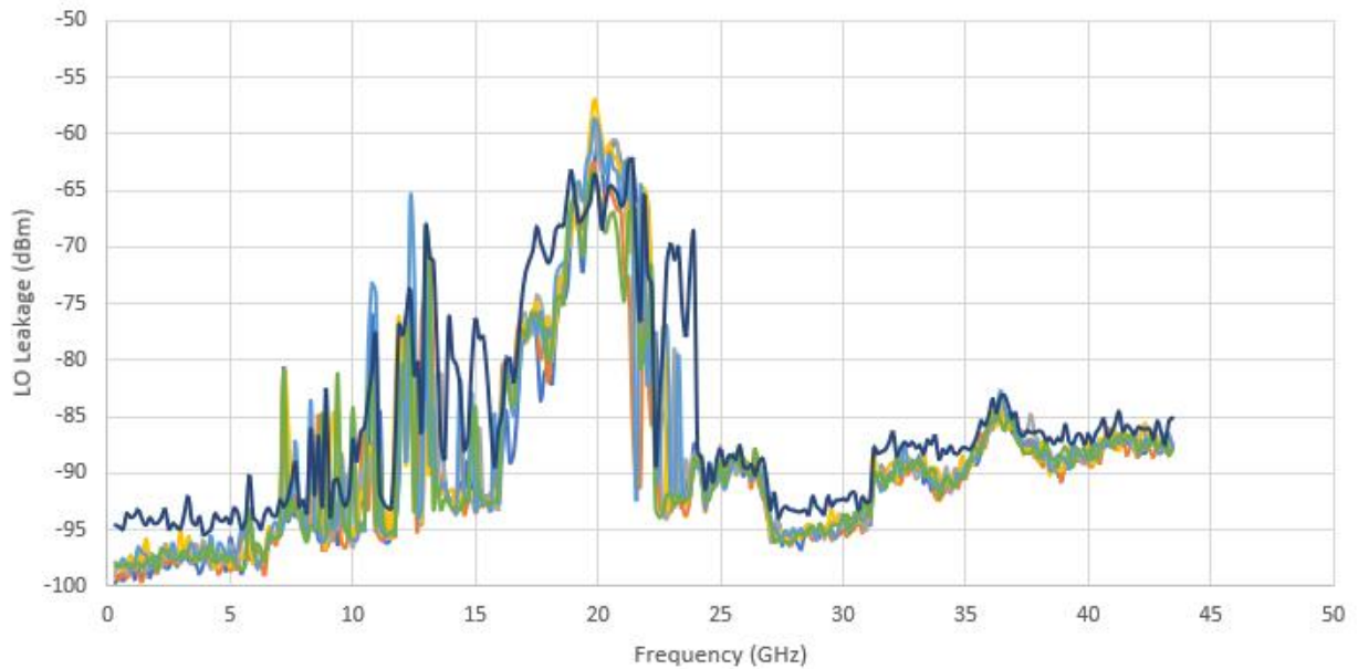
Typical LO Leakage (maximum sensitivity, -20 dBm reference level)
