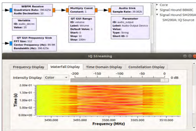
The GNU Radio application running the SM200B analyzer as a flowgraph block.
