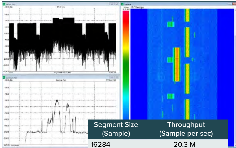
160 MHz looking at the entire 2.4 GHz ISM band
